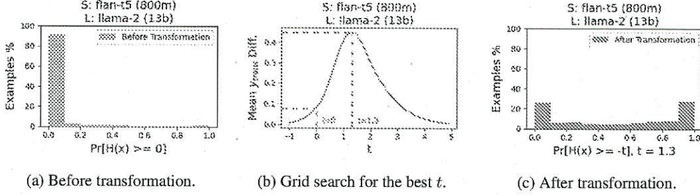
Figure 4: Effect of data transformation on labels for training the router.
